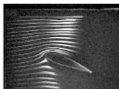
Figure 4. (12 MB, Quicktime movie) Animation of smoke particles flowing along a lifting aerofoil section.
